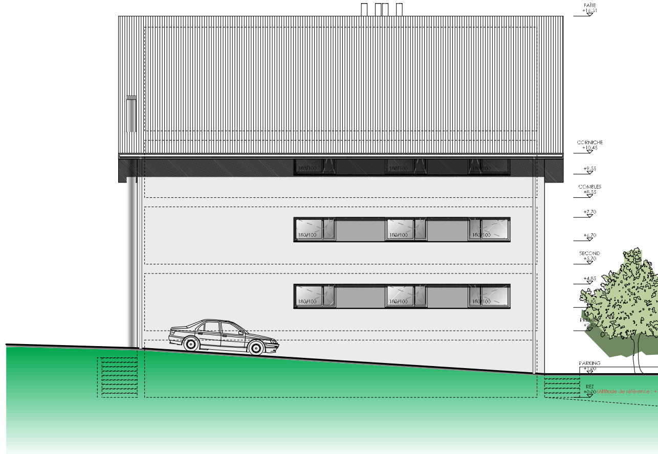
FACADE NORD (ELEVATION ARRIERE)
